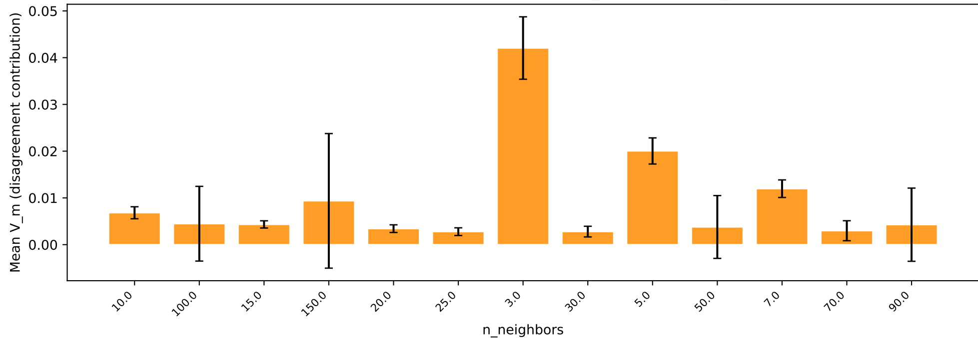
german — kNN: marginal effect of n_neighbors on V_m
