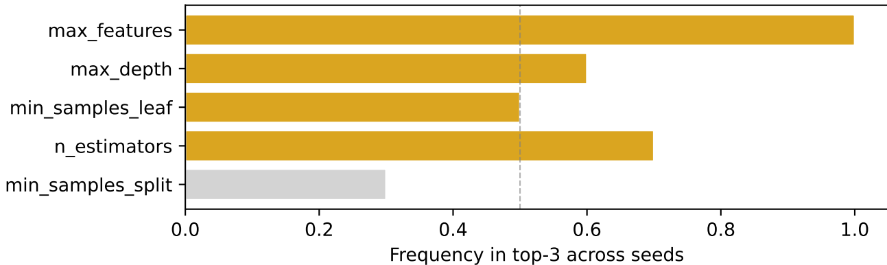
adult — RF: rank stability (top-3 frequency)
