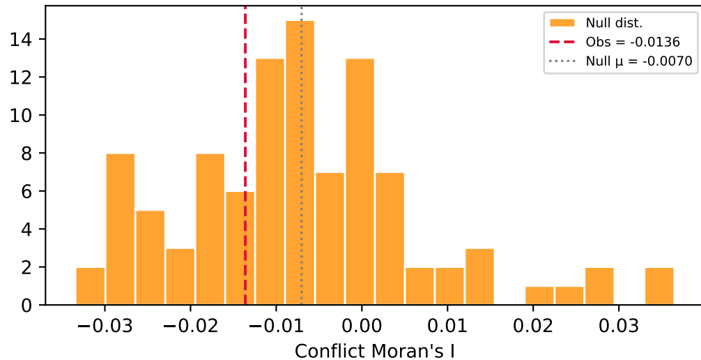
Conflict Moran's I (p_emp=0.723)
