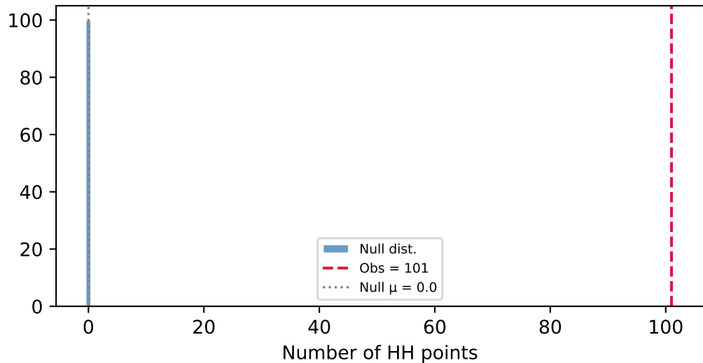
HH count (p_emp=0.010)
