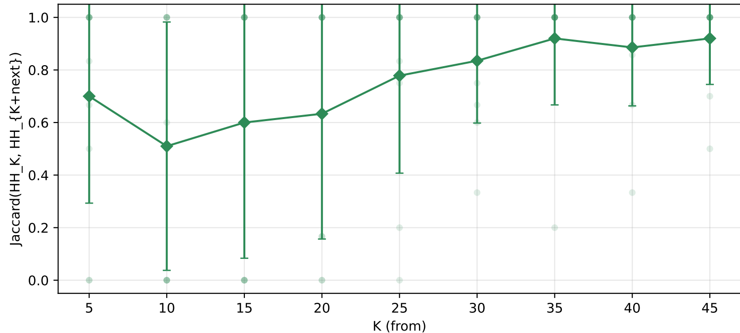
HH Jaccard between consecutive K — german
