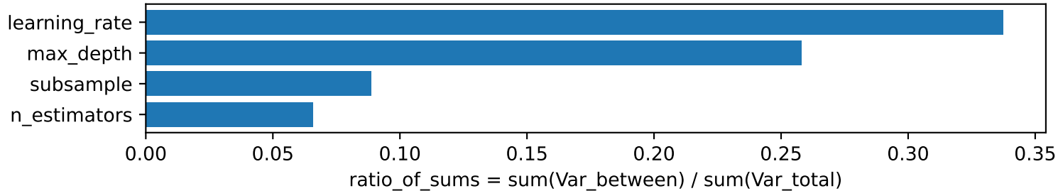
compas | seed=0 — GBM: top hyperparameters (within-family)
