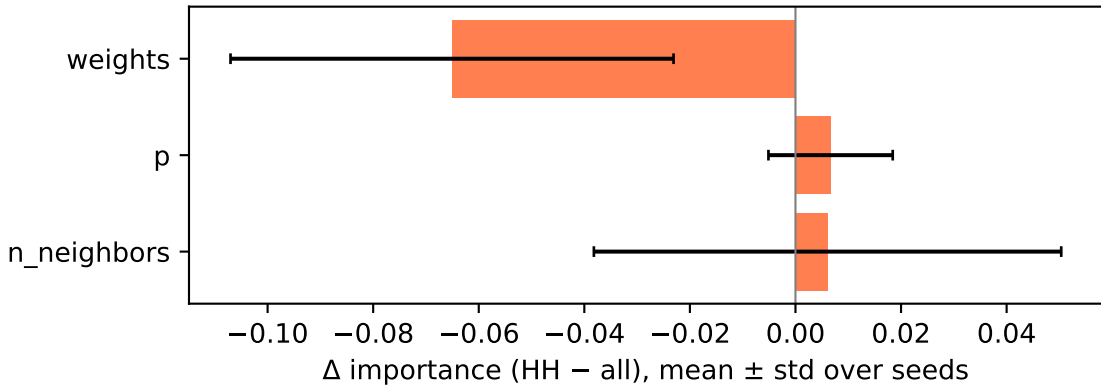
compas — kNN
