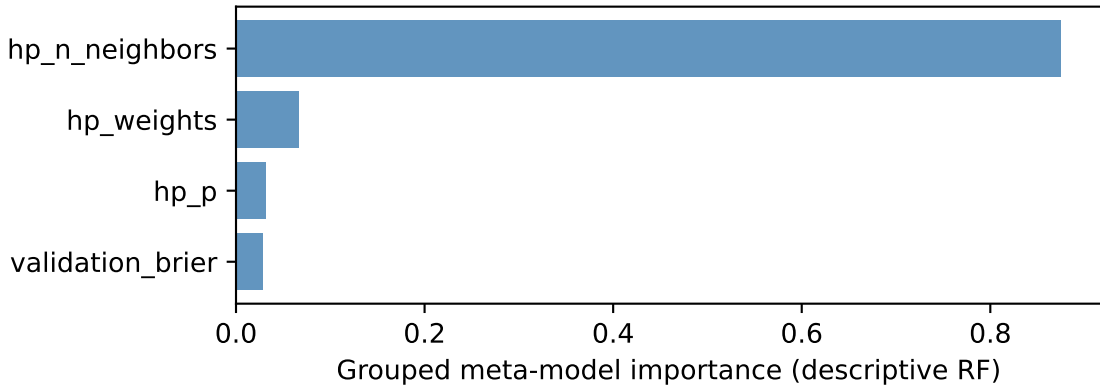
adult — kNN — Rashomon
