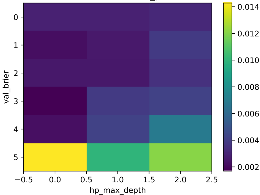
adult — GBM — full_pool
