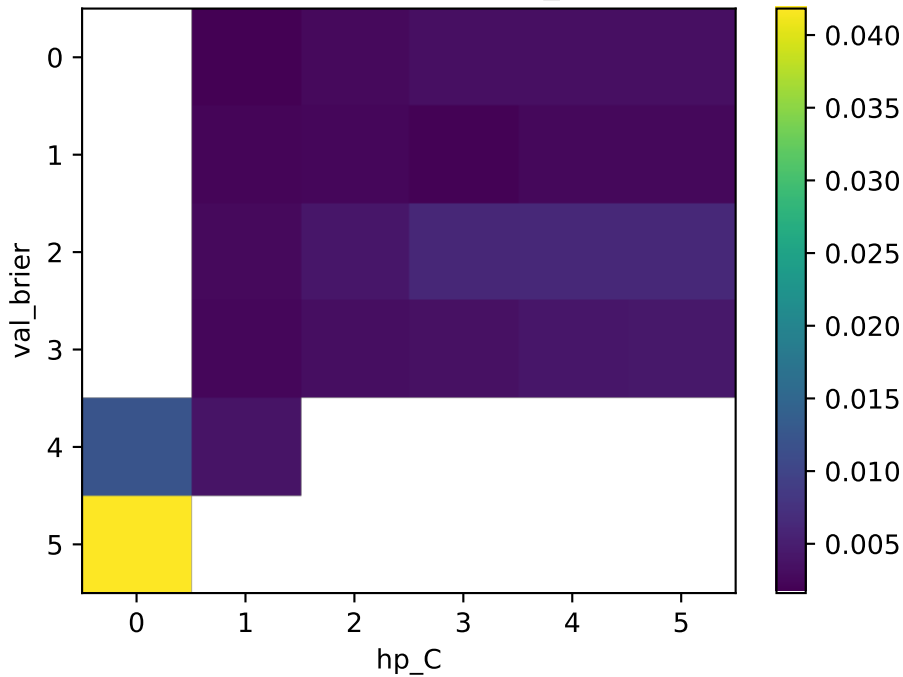
adult — LogReg — full_pool
