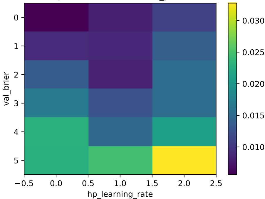
german — GBM — full_pool
