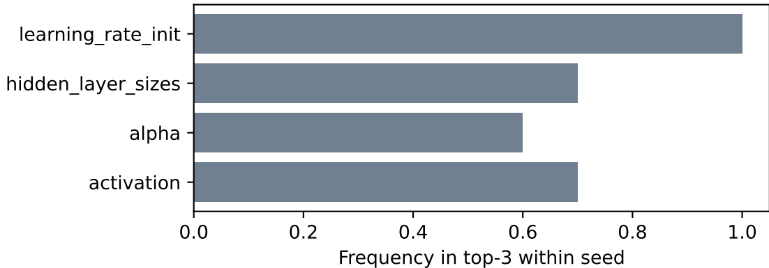
adult — MLP: rank stability (V_m importance, subset=all)
