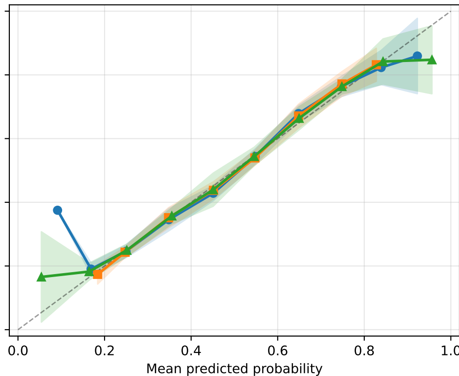
MLP (mean n=9.5)
