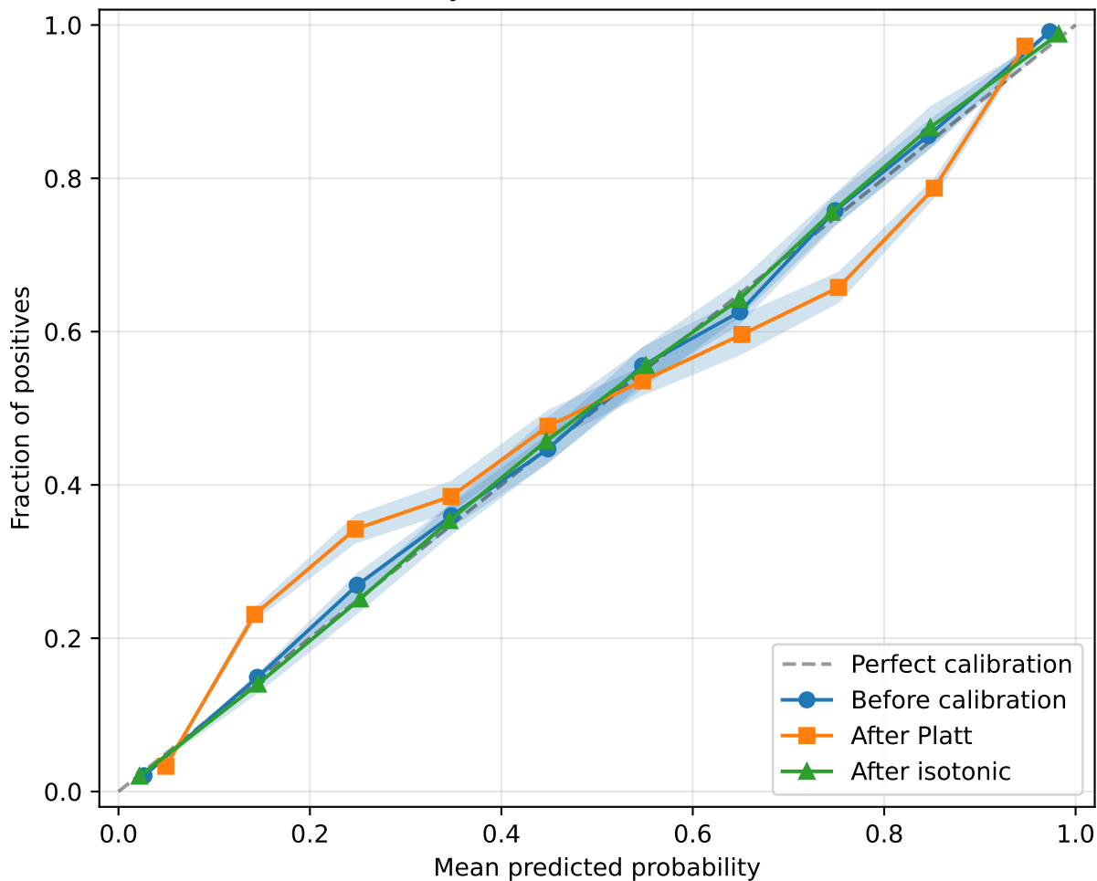
Reliability curves across runs — adult
