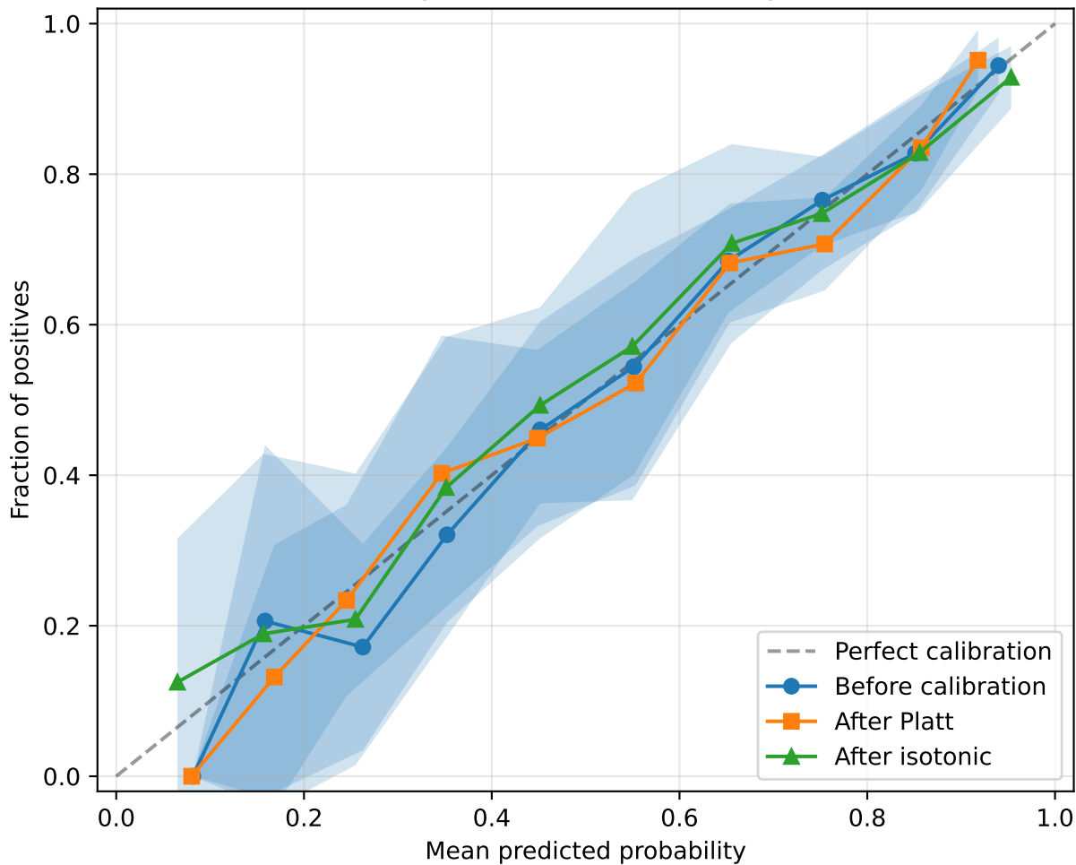
Reliability curves across runs — german
