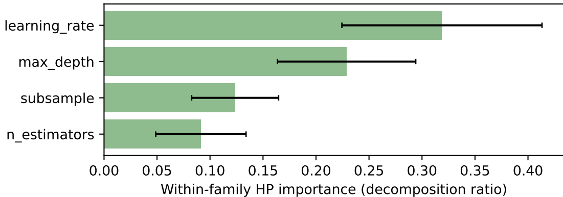
german — GBM — subset=all
