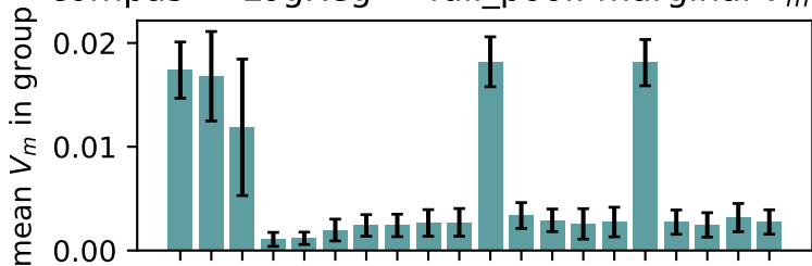
compas — LogReg — full_pool: marginal V_m by C
