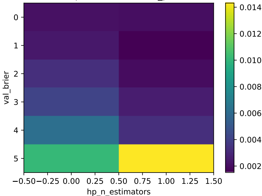
compas — GBM — full_pool
