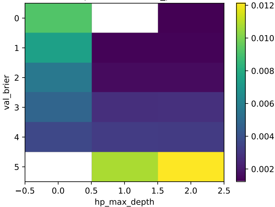
compas — RF — full_pool
