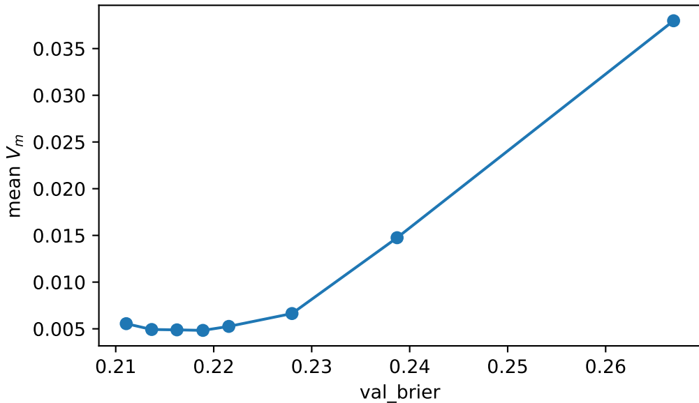
compas — kNN — Rashomon
