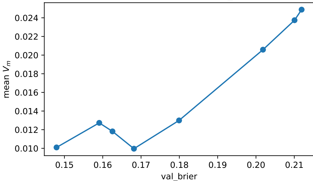
german — LogReg — full_pool
