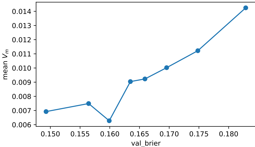
german — MLP — Rashomon
