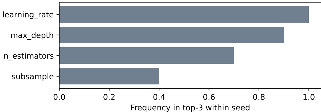
adult — GBM: rank stability (V_m importance, subset=all)
