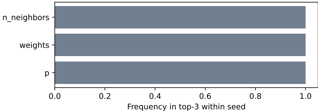
compas — kNN: rank stability (V_m importance, subset=all)
