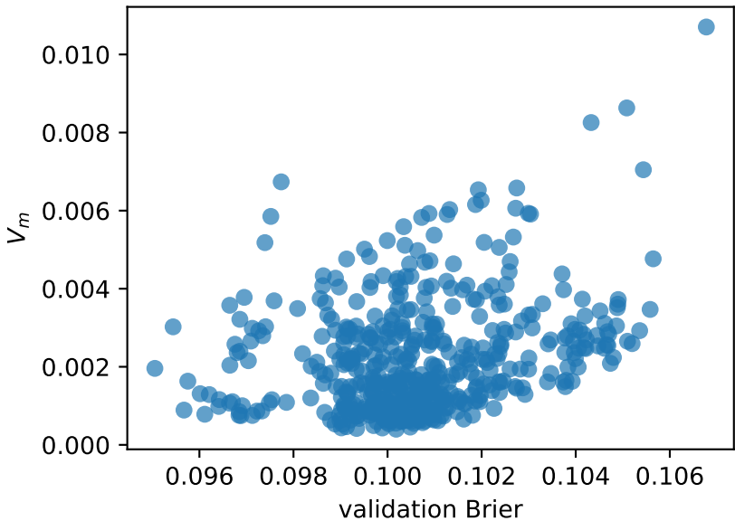
adult — MLP — full_pool
