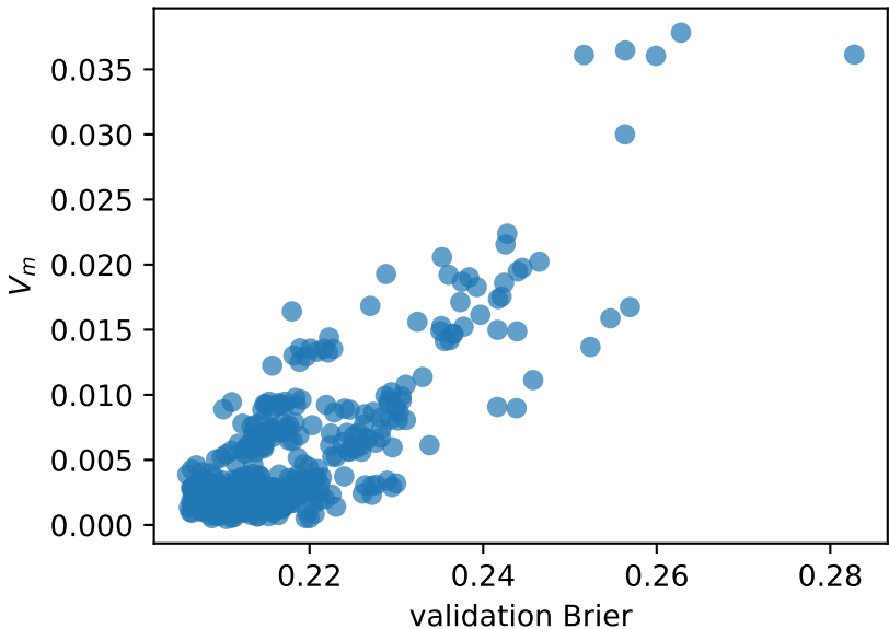
compas — GBM — full_pool
