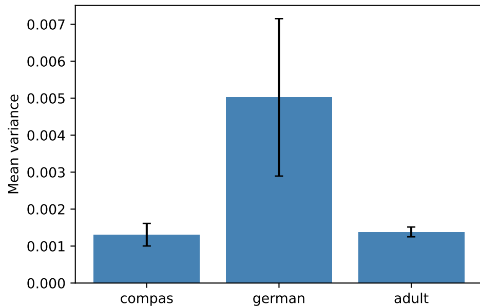
Mean variance (mean \pm std)
