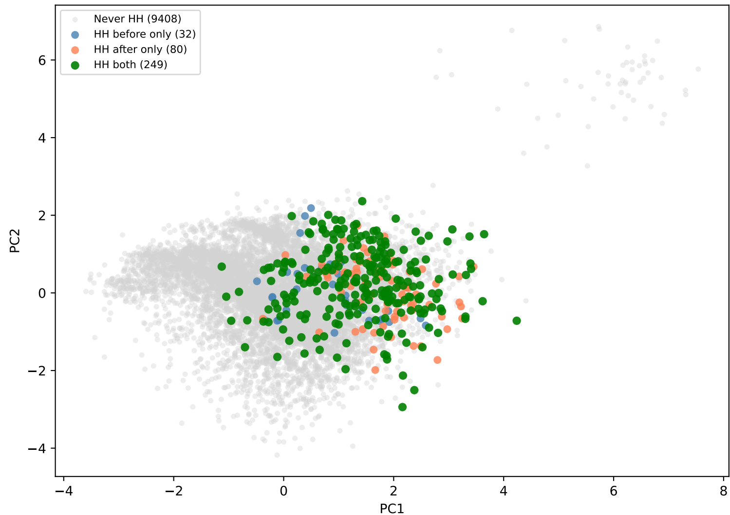
HH movement: before vs after isotonic calibration — adult (seed=5)
