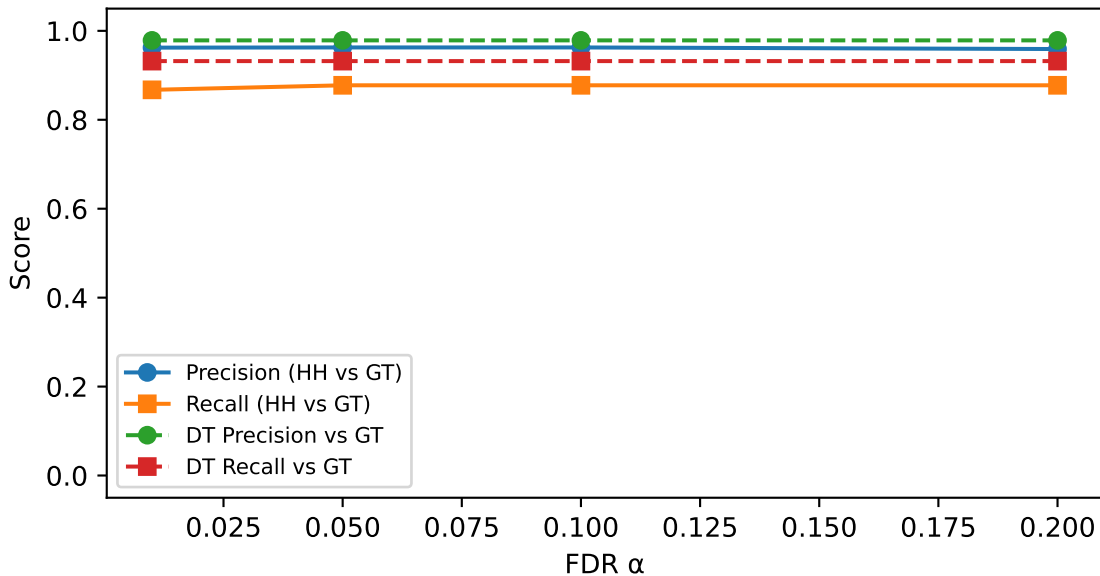
Precision & Recall vs \alpha (three islands)
