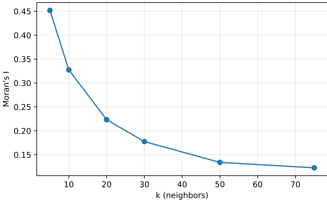
Spatial correlogram — compas (seed=2)
