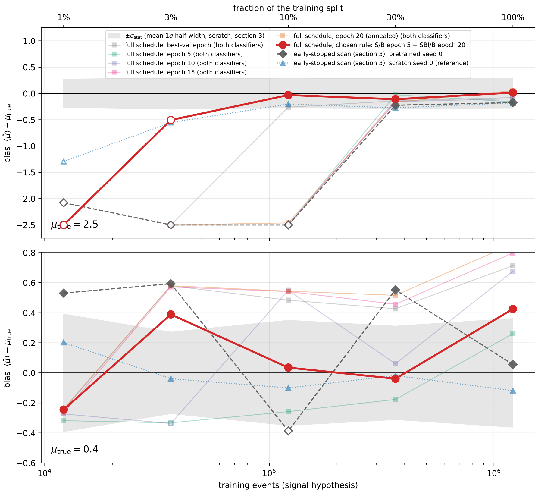
Fine-tuned pretrained EveNet, full 20-pass schedule: bias vs training statistics (48 weighted toys, 300 fb -1 , seed 0)
