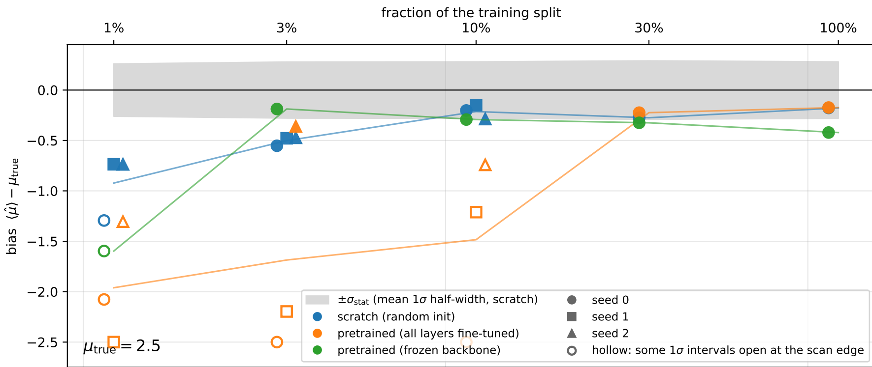
NSBI signal-strength bias vs training statistics, every seed shown (48 weighted toys, 300 fb -1 )
