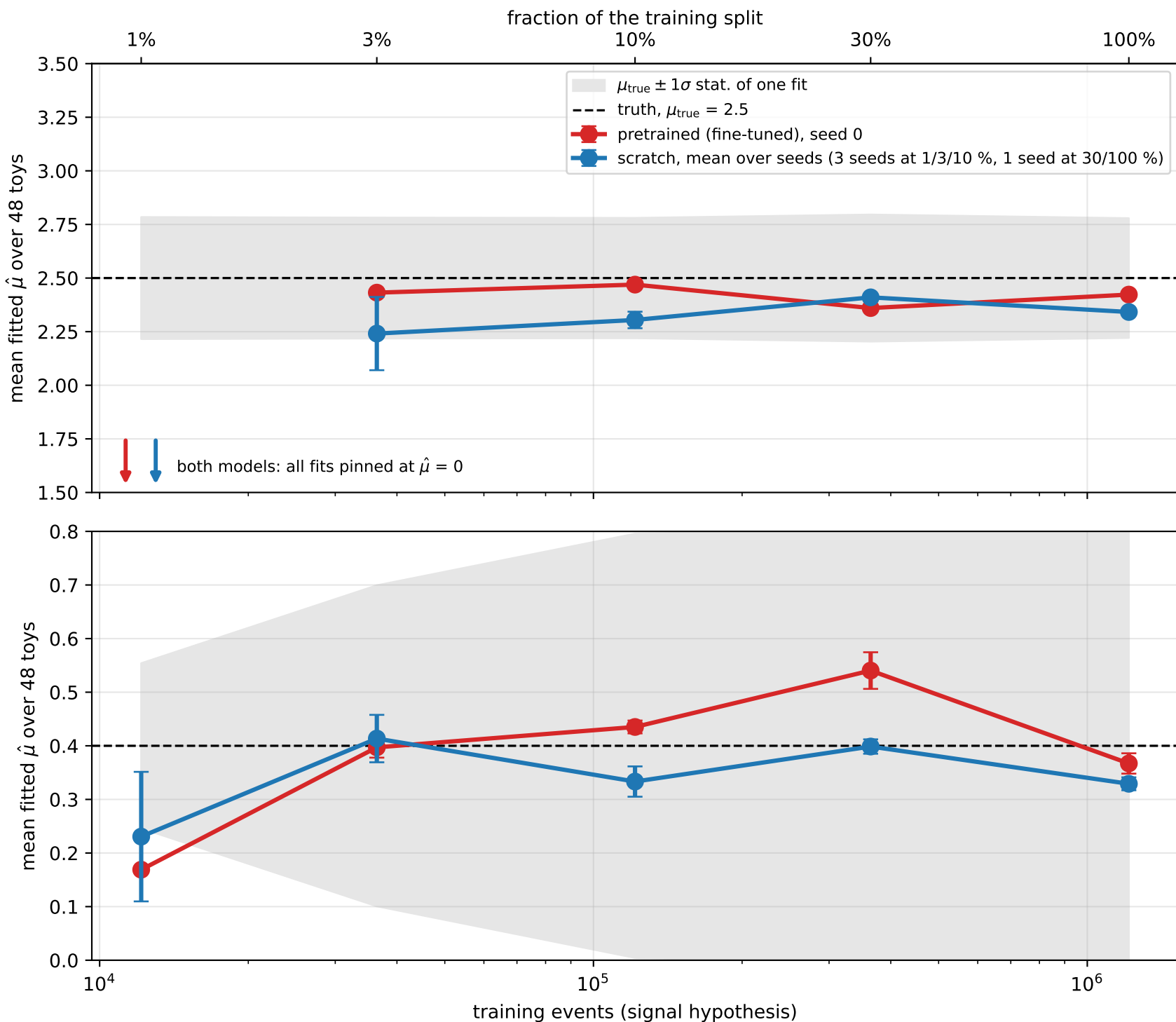
Fitted signal strength vs training statistics: pretrained vs scratch (48 toys, 300 fb -1 )
