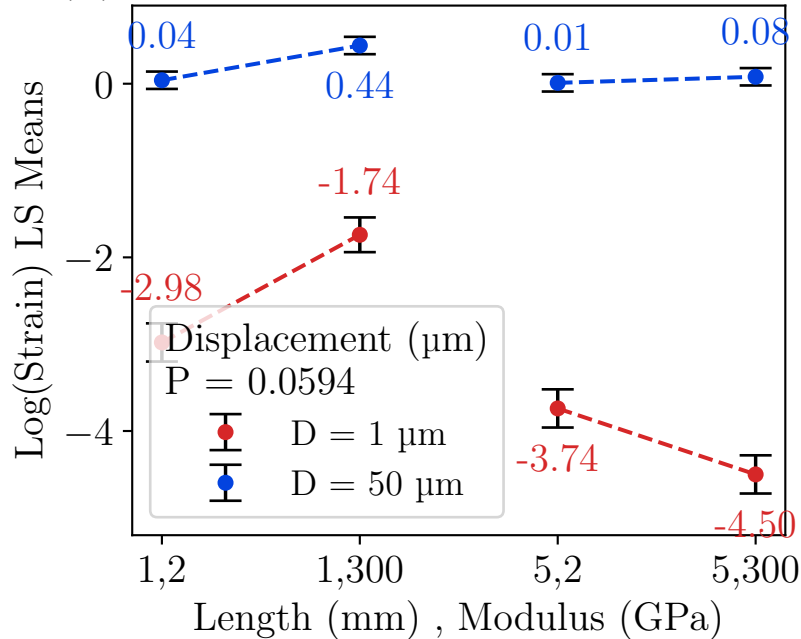
(b) Length \times Modulus \times Displacement
