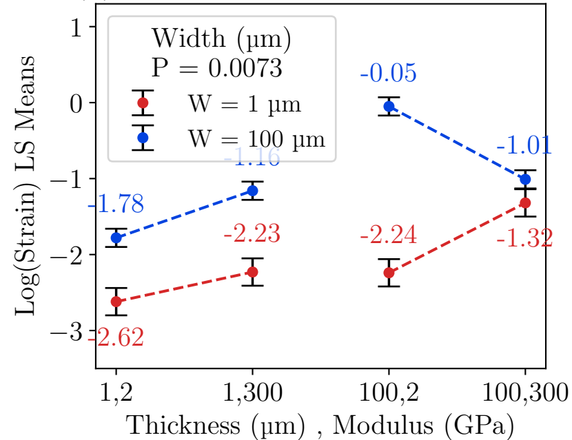
(a) Thickness \times Modulus \times Width
