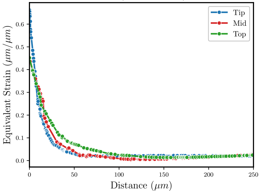
Equivalent Strain (Tip–Mid–Top) of the MEA
