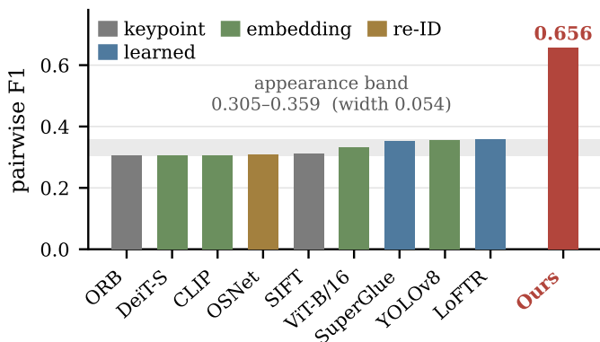
Fig. 1. The appearance ceiling. Pairwise F_1 for nine crop-scope matchers spanning four method families on CRACKID test. Every method falls inside the band 0.305–0.359 — width 0.054 — pressed against the 0.305 chance floor ( 2p/(1+p) for this pool), irrespective of family, era, or compute budget. The geometric reference baseline (red) leaves the band. Ranking metrics separate the same methods over a 0.30 range; the decision metric does not.
