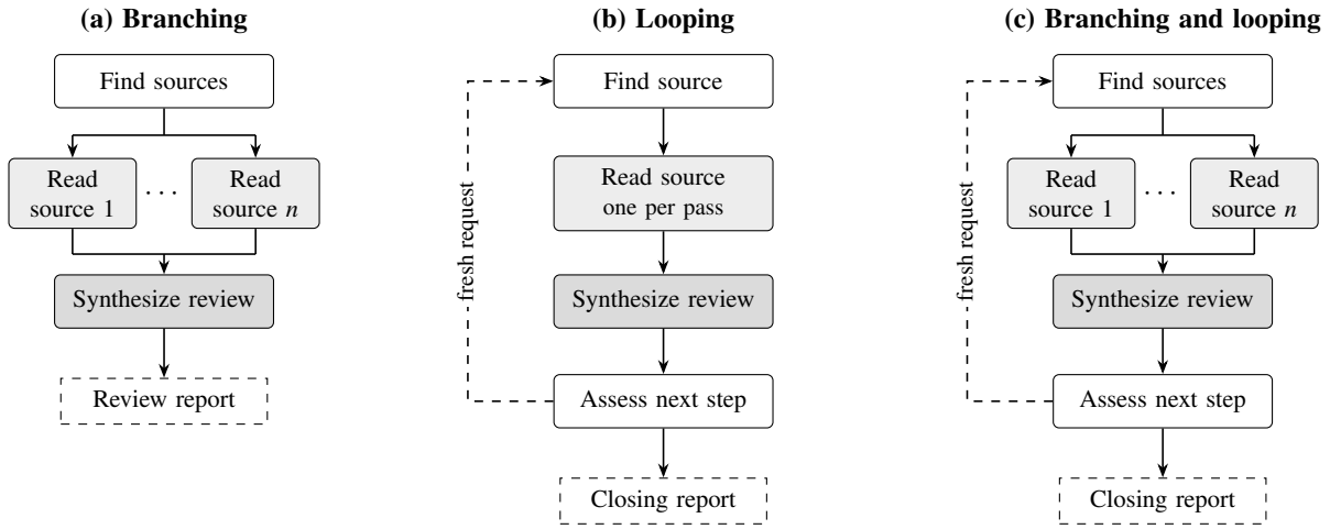
Figure 1: Session patterns specified by three literature-review FAMs. Each rounded box represents an agent session invoking the named operation. In (a) and (c), there is one reading session per selected source; the ellipsis leaves the source count unspecified. These sessions invoke the same Read source schema. Solid arrows show principal artifact dependencies. Dashed return arrows indicate new passes enabled by fresh requests; dashed rectangles are output artifacts.
