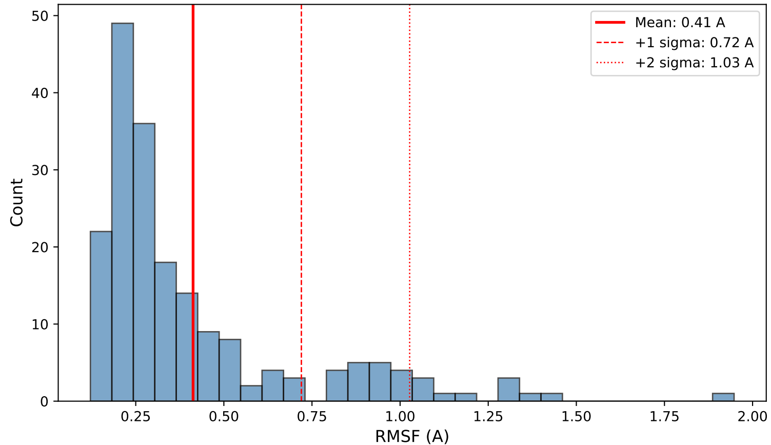
Distribution of Per-Residue RMSF
