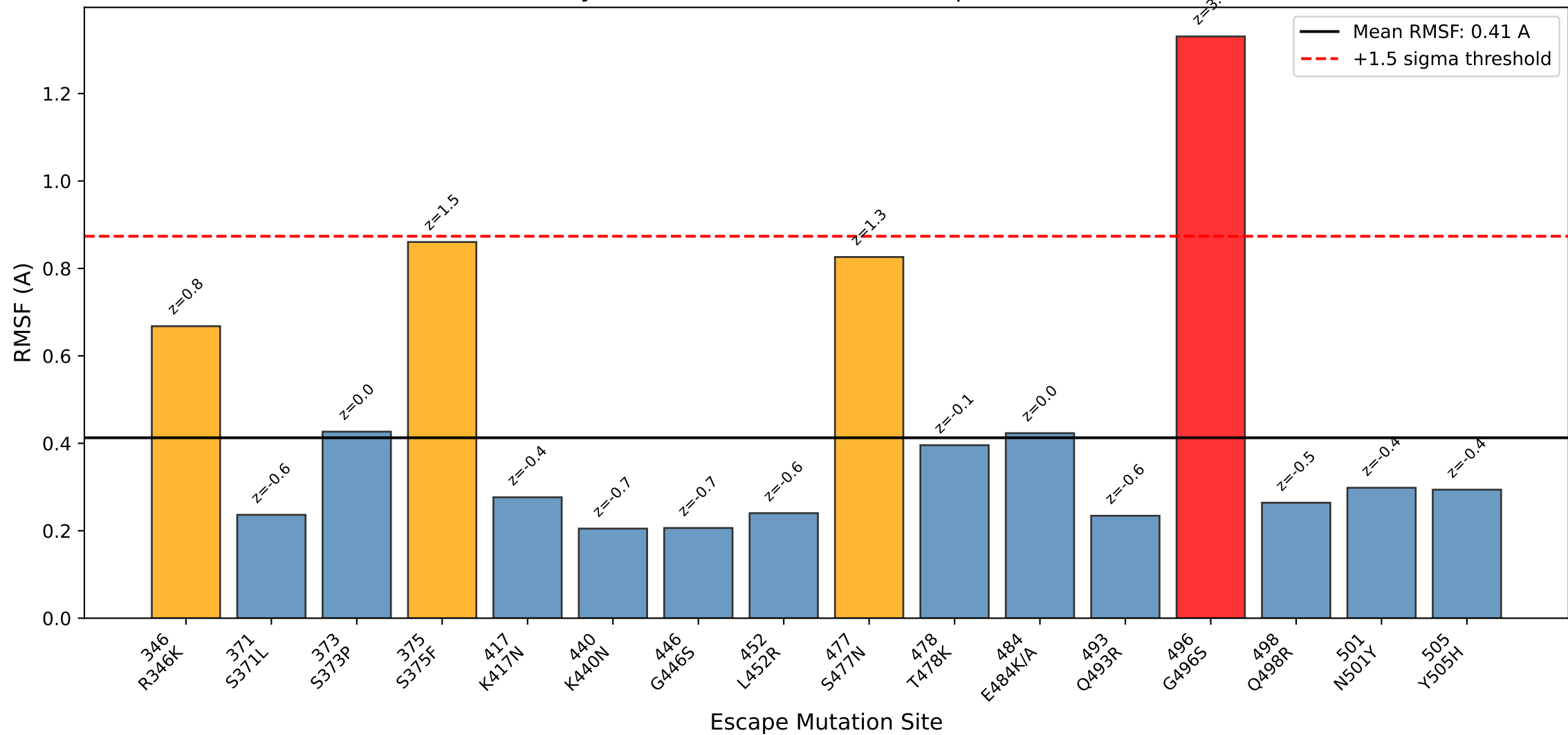
Flexibility at Known SARS-CoV-2 Escape Mutation Sites
