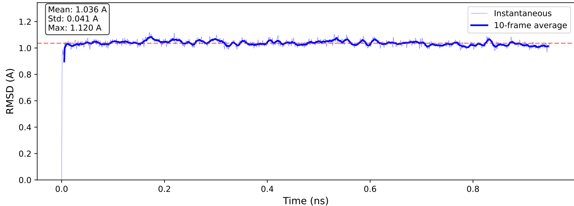
Backbone RMSD from Initial Structure
