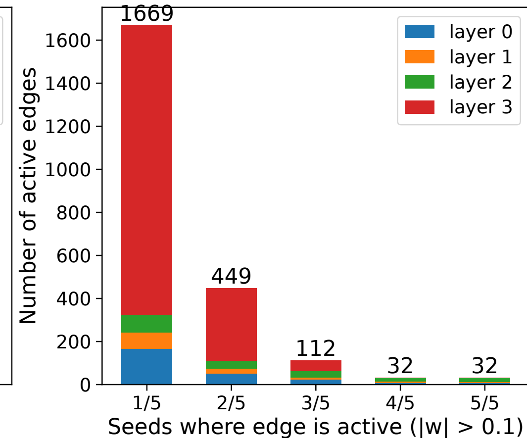
Active soft-link consistency (|w| > 0.1, 5 seeds)
