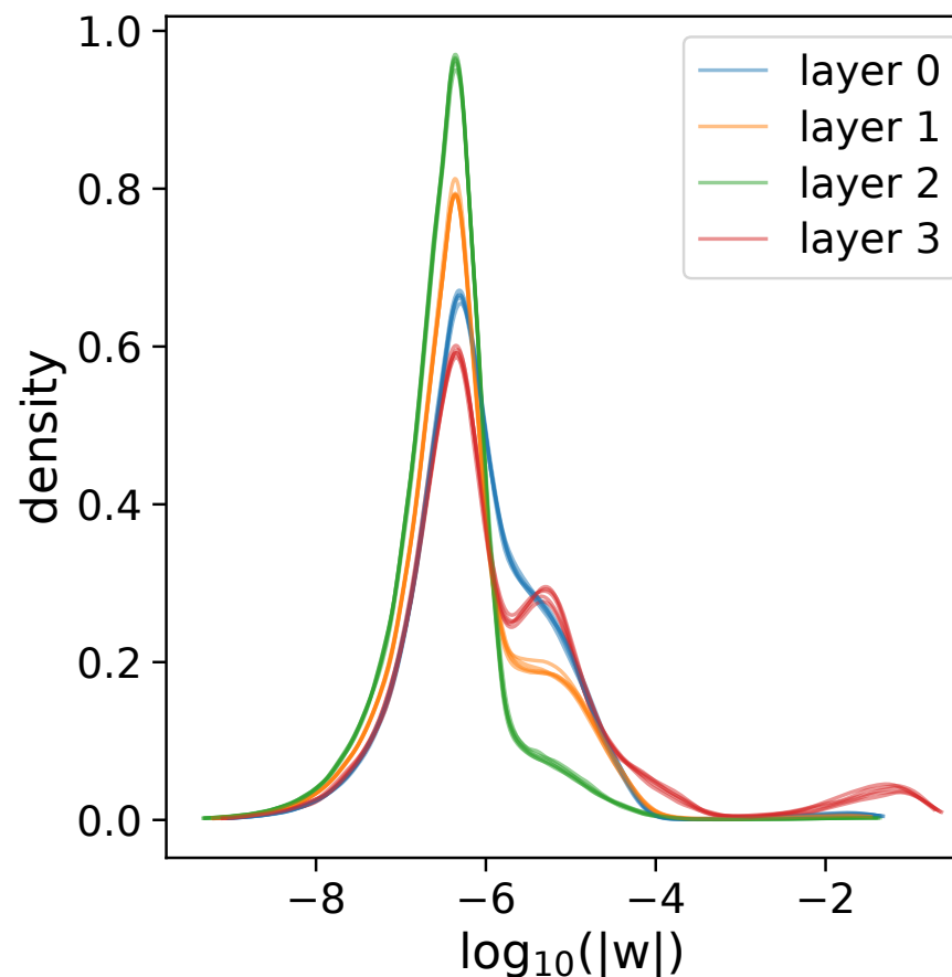
Weight magnitude distribution per layer (all seeds overlaid)
