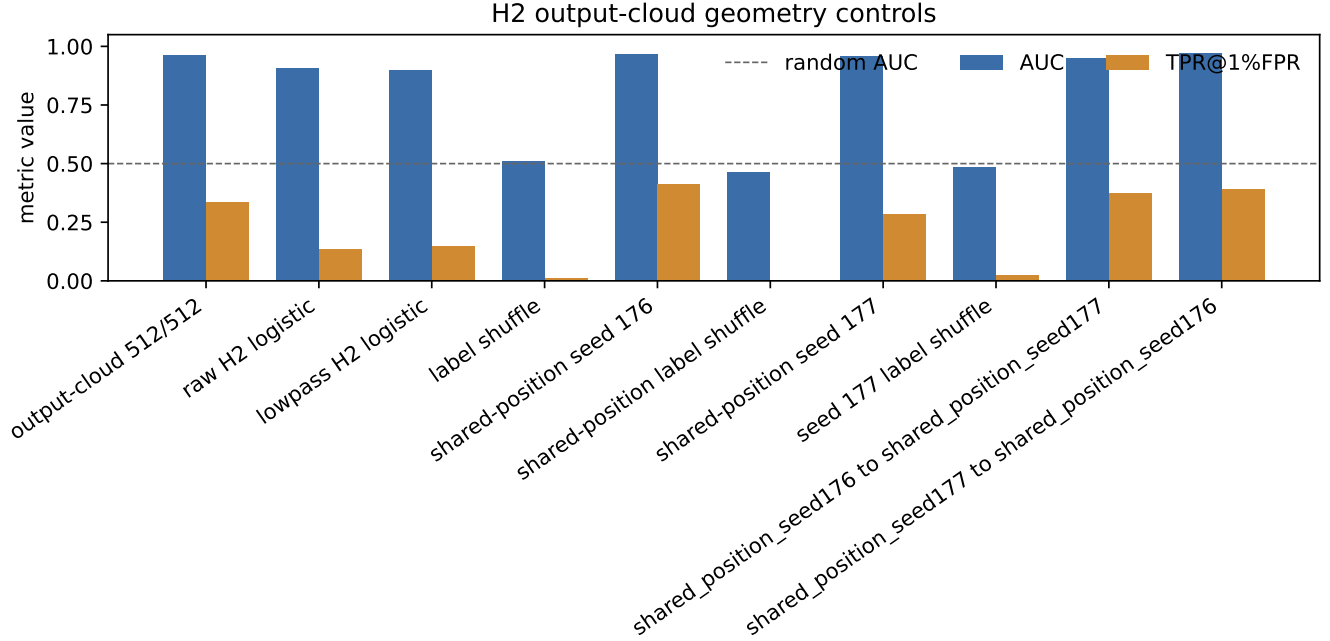
Fig. 4. H2 output-cloud geometry controls. The signal beats raw/lowpass baselines and survives label-shuffle, seed-offset control, seed stability, and cross-cache transfer. It remains a research candidate because portability to the SD/CelebA img2img contract is weak or not distinct from simple distance.
