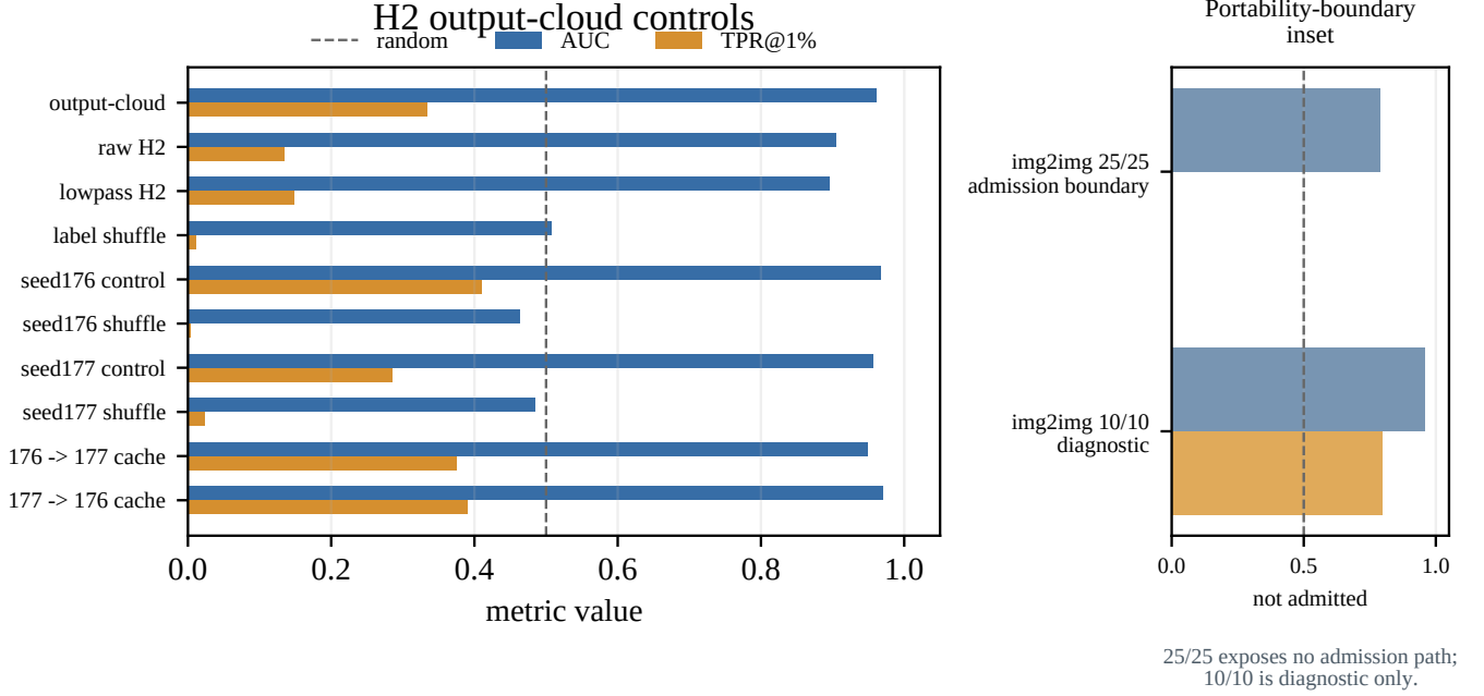
Fig. 6. Candidate-side admission stress test for H2 output-cloud geometry. The H2-family metric is above chance and stays candidate-only: it collapses under label shuffle and persists under seed-offset control, seed stability, and same-family cache-reuse checks. SD/CelebA img2img portability rows are shown as a boundary inset: the 25/25 packet leaves the admission path absent, and the 10/10 row is diagnostic only.
