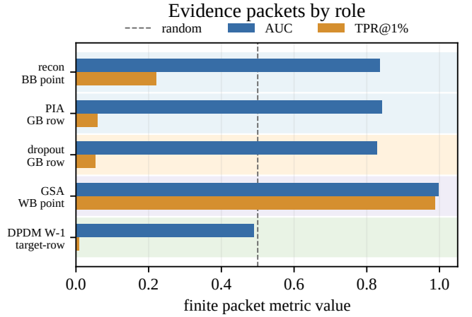
Fig. 5. AUC and TPR@1%FPR for role-separated worked-example cases. Rows are ordered by access and allowed claim role, and each label includes its replay tier. The figure catalogues role-separated evidence; benchmark ranking and replay-derived intervals are outside this display.
