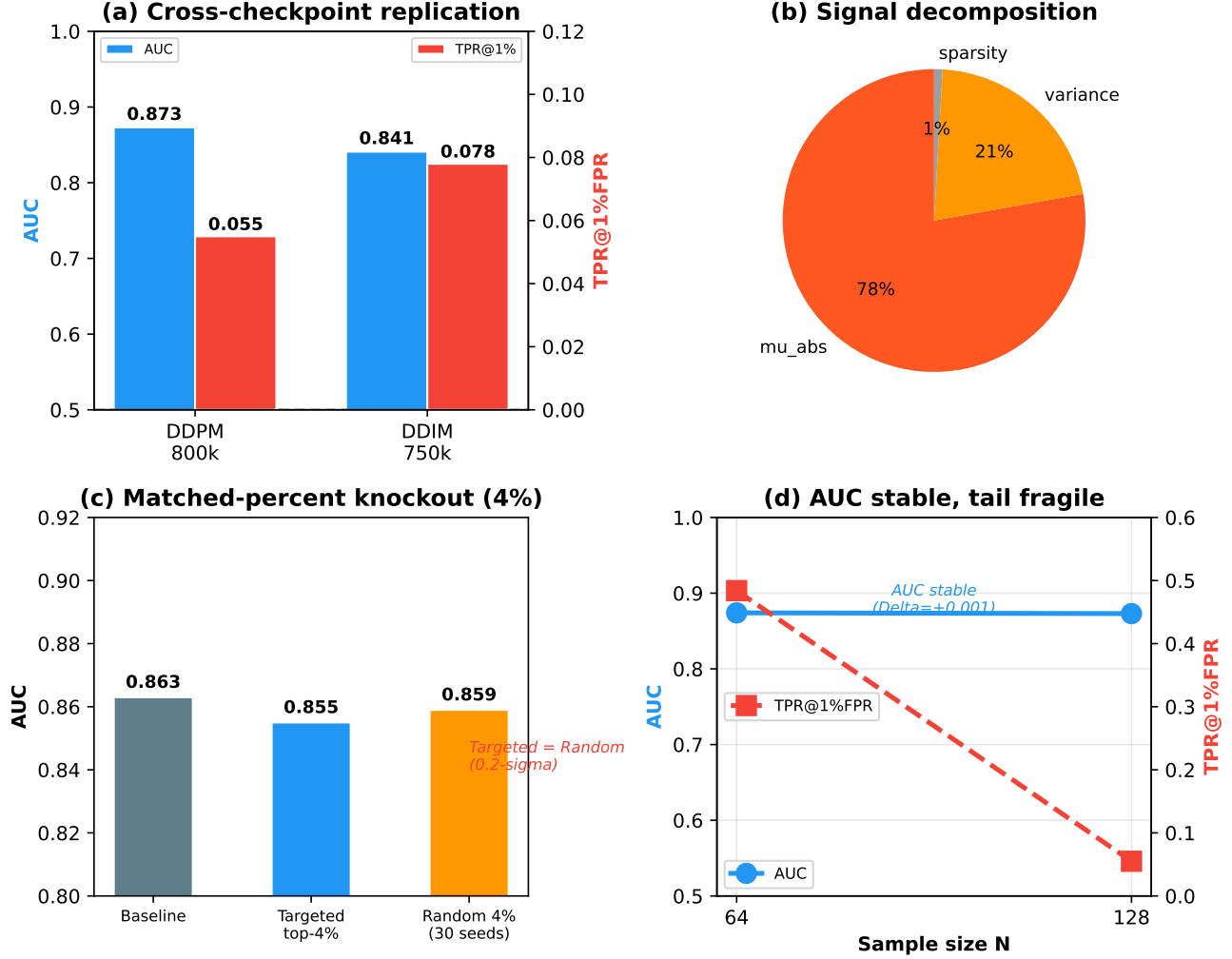
Fig. 4. H1 Distributed Activation-Amplitude Bias. (a) Cross-checkpoint replication: AUC remains 0.84–0.88 across DDPM 800k and DDIM 750k. (b) Signal decomposition: activation magnitude ( \mu_{\text{abs}} ) carries 78% of LR coefficient mass. (c) Matched-percent knockout: neither targeted top-4% nor random 4% deletion meaningfully reduces AUC, confirming distributed redundancy. (d) AUC stays stable under scale-up while TPR@1%FPR collapses, demonstrating the gap between aggregate separability and forensic admissibility.
