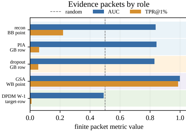
Fig. 6. AUC and TPR@1%FPR for role-separated worked-example cases. Rows are ordered by access and allowed claim role, and each label includes its replay tier. The figure catalogues role-separated evidence; benchmark ranking and replay-derived intervals are outside this display.
