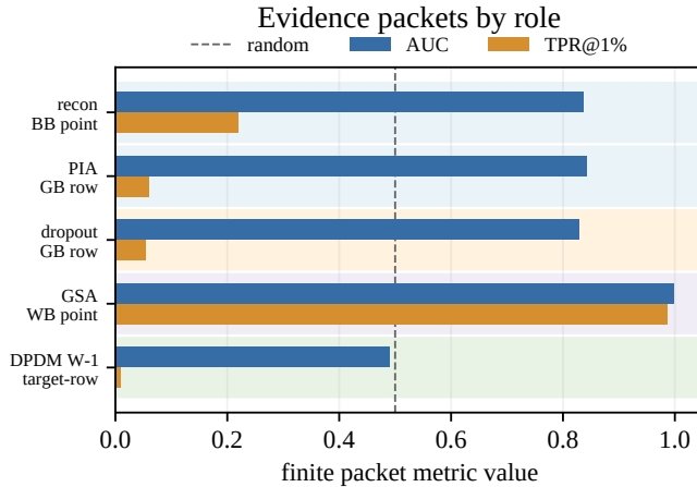
Fig. 4. AUC and TPR@1%FPR for role-separated worked-example cases. Rows are ordered by access and allowed claim role, and each label includes its replay tier. The figure catalogues role-separated evidence; benchmark ranking and replay-derived intervals are outside this display.
