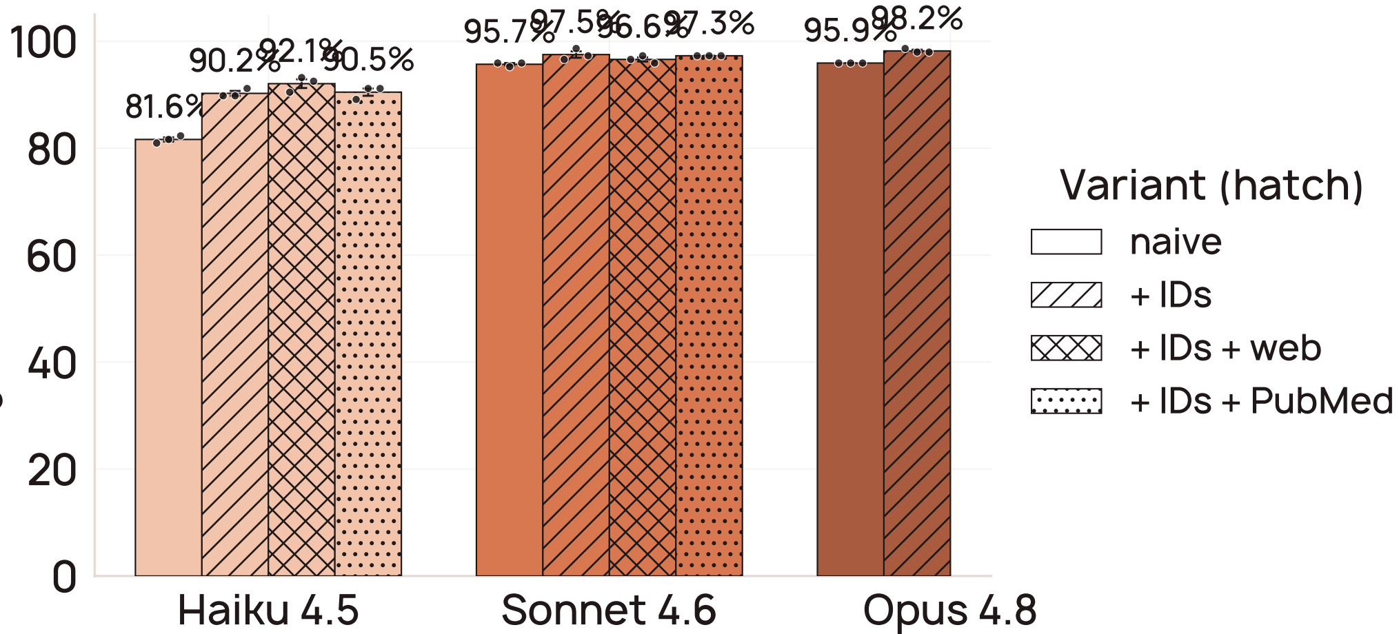
Overall accuracy on 147-gene benchmark
