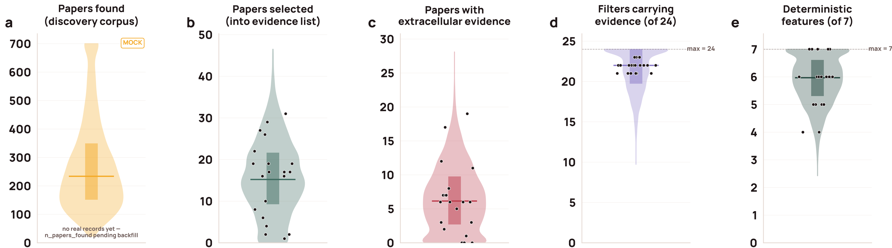
Each panel: per-gene distribution on one richness axis. Dark dots = real values from the 20 published deep dives. Violin shape + IQR box = synthesised 5,000-draw fan extrapolating to a full cohort (lognormal for papers_found around the methods-documented median 234.5 / range 50–400; Gaussian around the empirical mean \pm std (or 15%% mean, whichever larger) for the other axes). MOCK pending the discover-only backfill for papers_found and the full cohort sweep.
