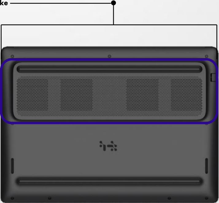
Cryo-Chamber structure on configurations with NVIDIA® GeForce RTX™ 5050 or 5060
