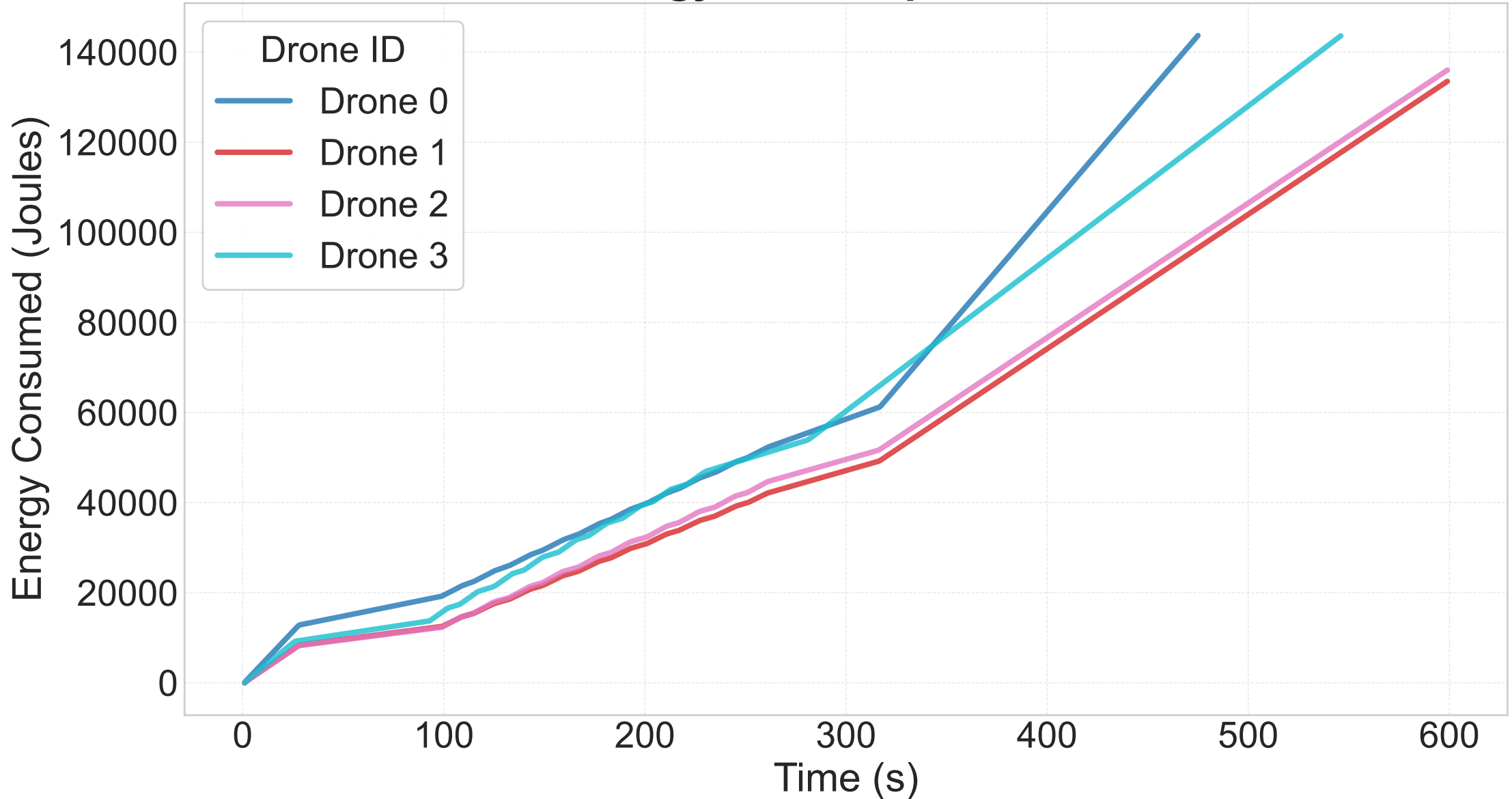
Total Energy Consumption Over Time
