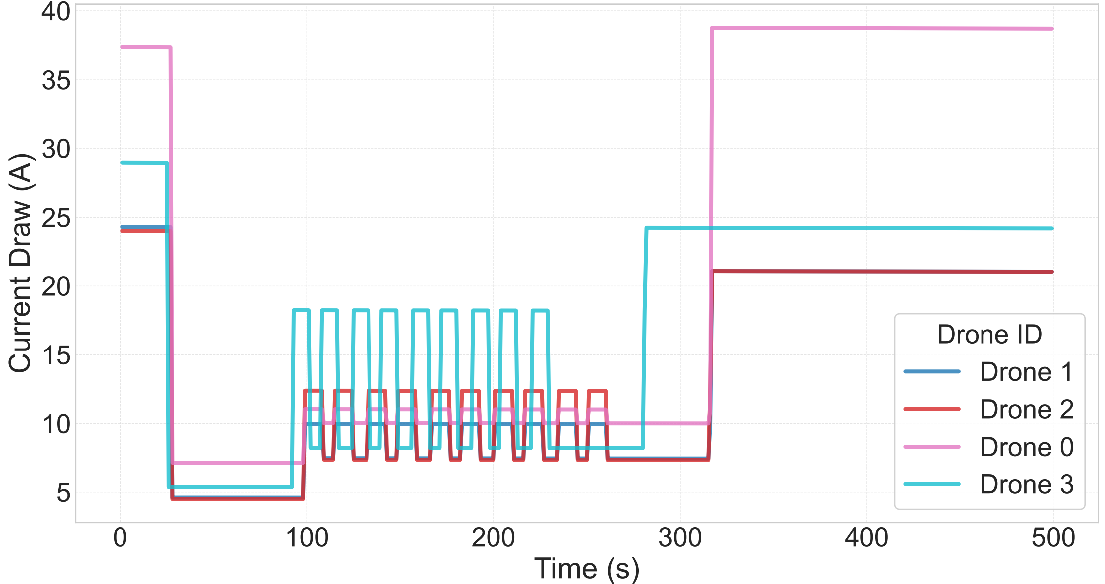
Instantaneous Current Draw Over Time
