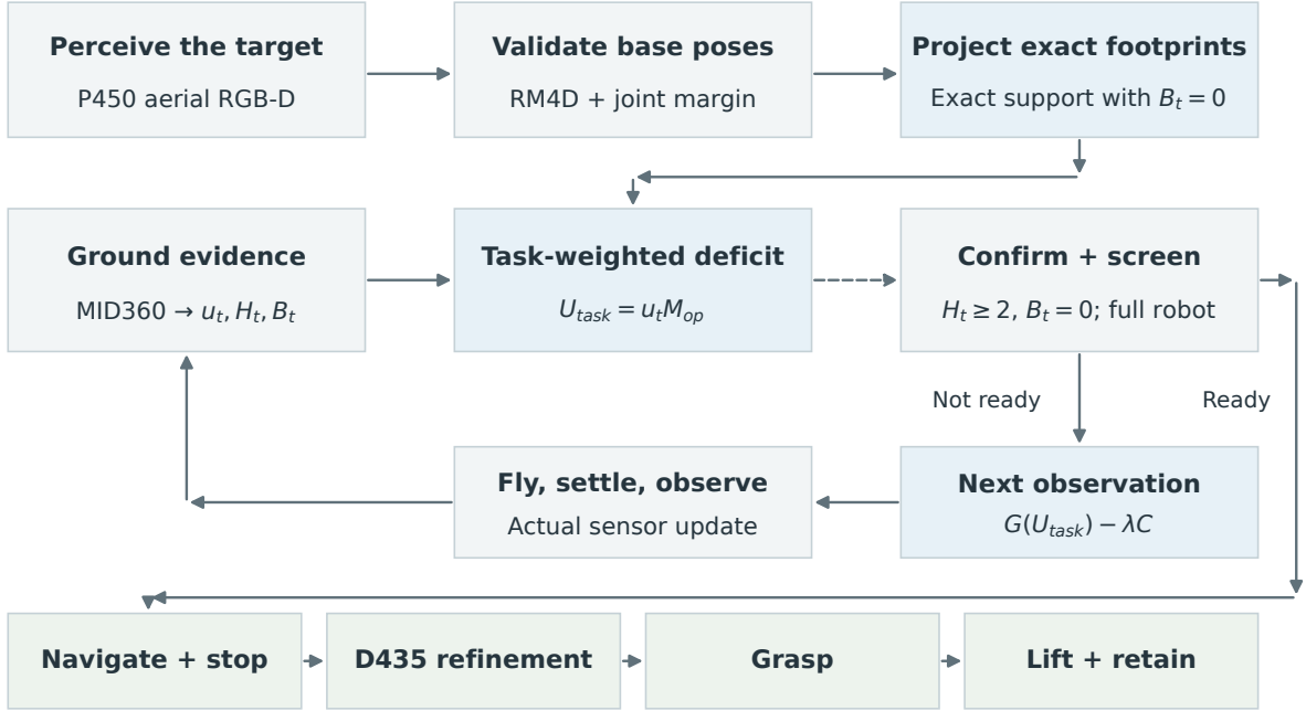
Figure 1: Manipulation-guided sensing and physical handoff. Validated exact base footprints project future manipulation requirements into environment space. Measured MID360 evidence supplies observation deficit and operational blocking; blue boxes highlight the relevance-weighted sensing path. The dashed connector denotes workflow order, not an input from deficit to confirmation: confirmation independently requires measured H_t and B_t . Full-robot screening precedes another view. A ready candidate enters the shared execution sequence (green), with D_{exec} checked after fresh D435 refinement. Further observation requires remaining budget and a positive admissible score; failure may terminate the task at any stage. This is a schematic, not a trial reconstruction.
