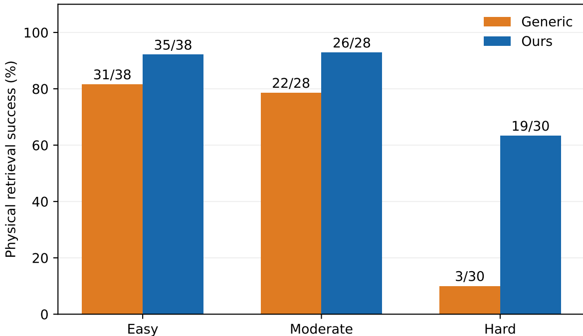
Same-version paired evaluation; tier outcomes are descriptive
